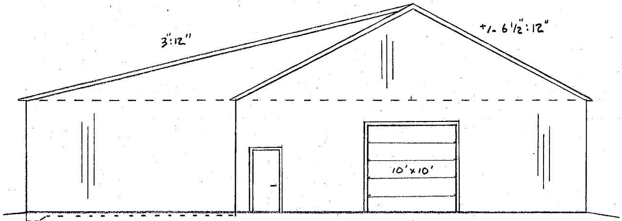
FRONT ELEV : \frac{3}{32}'' = 1'-0''
