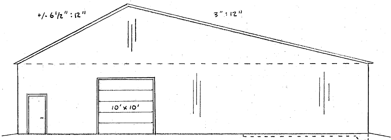
REAR ELEV : \frac{3}{32}'' = 1'-0''
